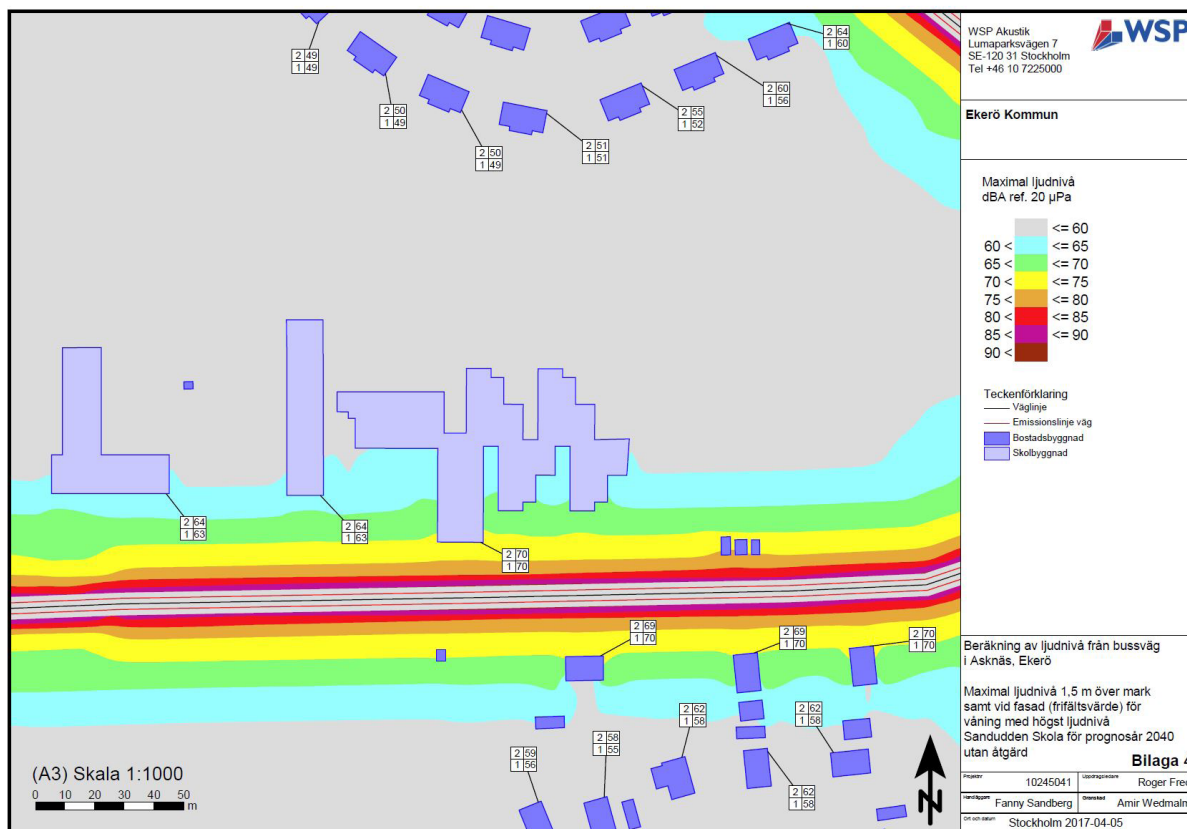
Figur 28, maximal ljudnivå dBA (WSP, 2017-04-05)
