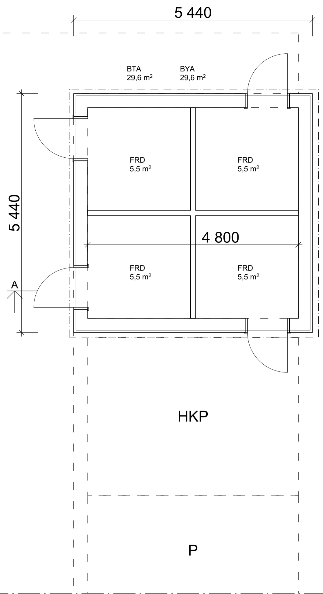
PLAN
